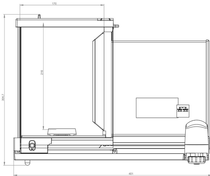
XA 52.5Y.M.A Microbalance
