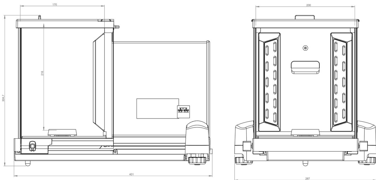
XA 53.5Y.M.A Microbalance
