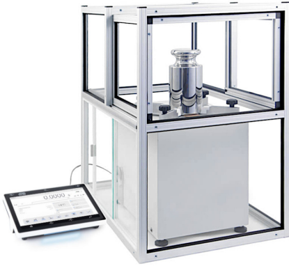
APP 10.5Y.KO Mass Comparator
