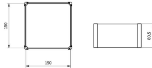
Draft shield for precision balances
