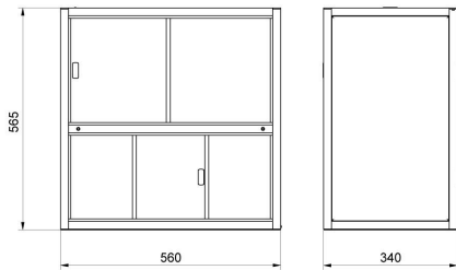
Anti-draft chamber for WAY-KO mass comparators
