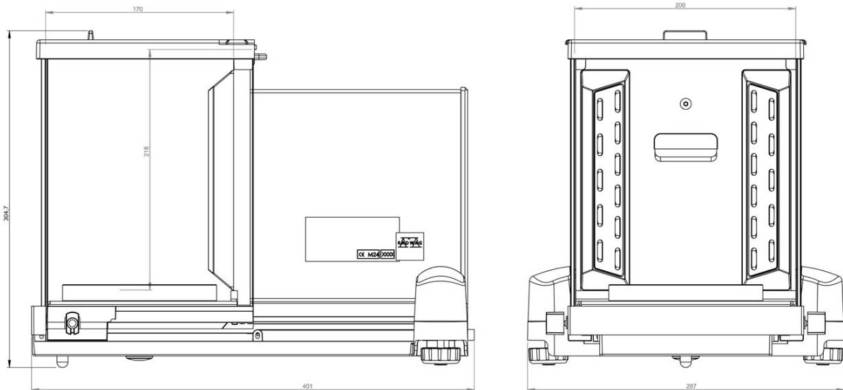
XA 110.5Y.A Analytical Balance
