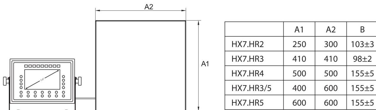
HR Platform
